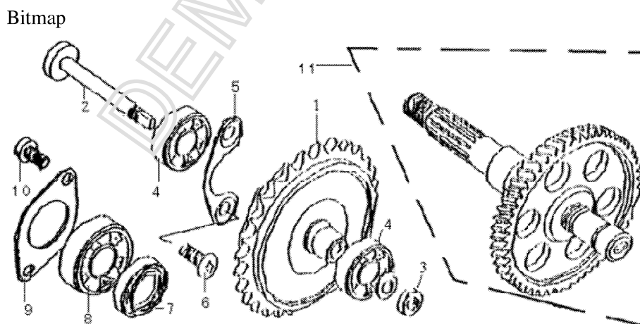
FIG.24 TRANSMISSION
