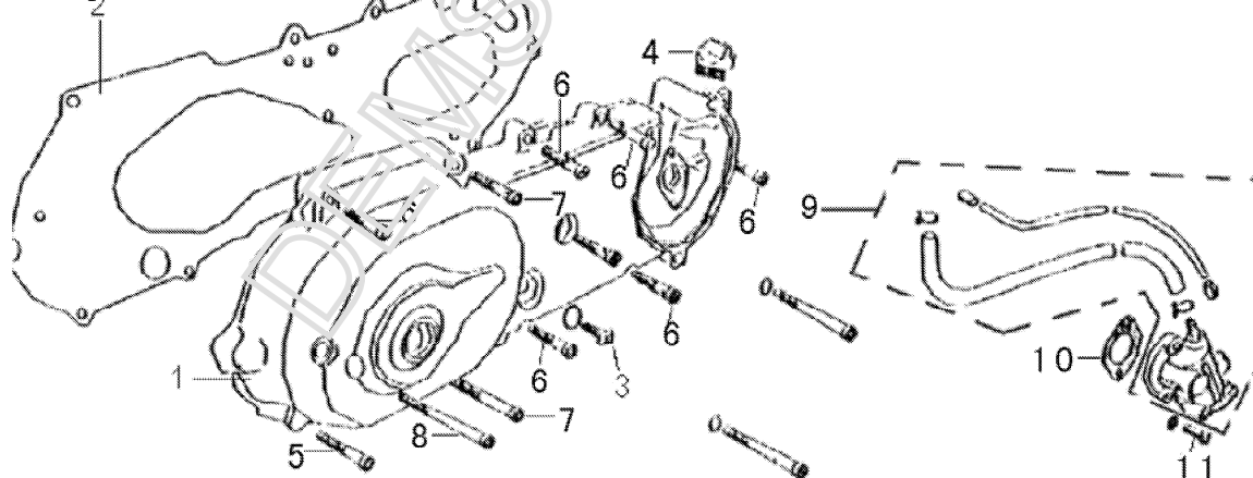
FIG.26 LEFT CRANKCASE COVER
