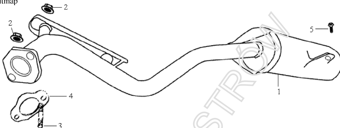
FIG.25 EXHAUST MUFFLER ASSY
