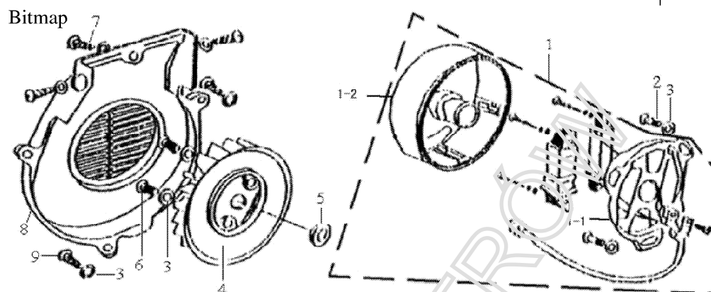
FIG.23 GENERATOR
