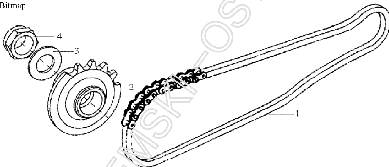
FIG.11 DRIVE CHAIN
