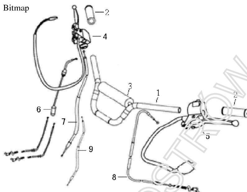
FIG.9 STEERING HANDLE, CABLE
