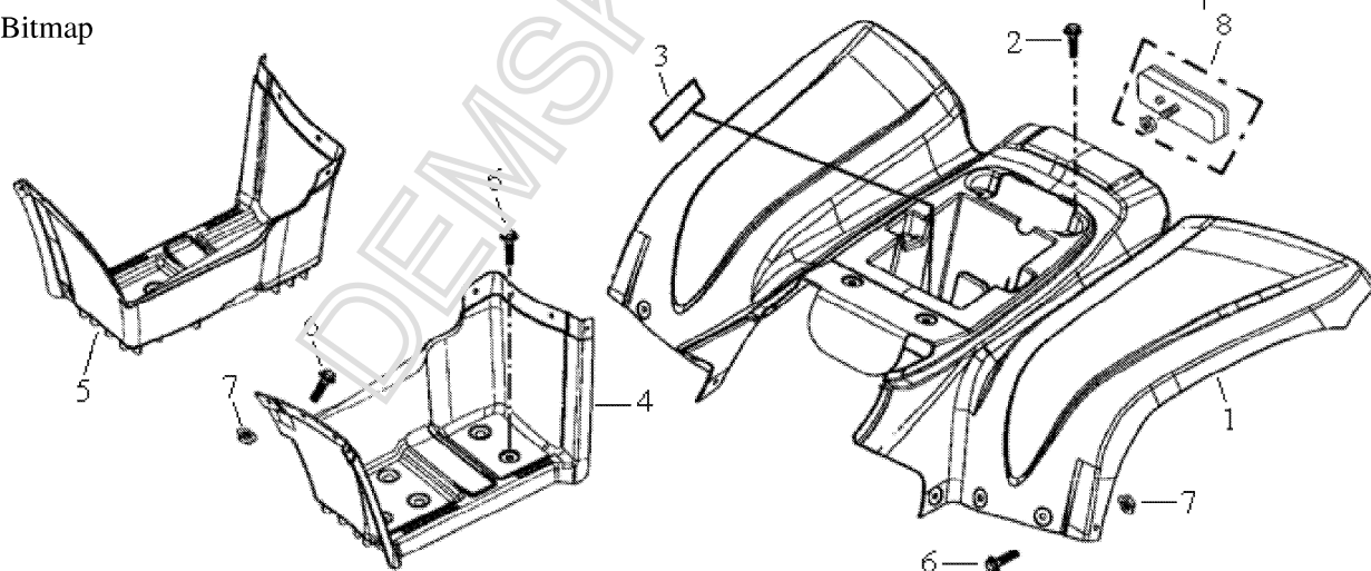
FIG.2 REAR FENDER, FOOT REST
