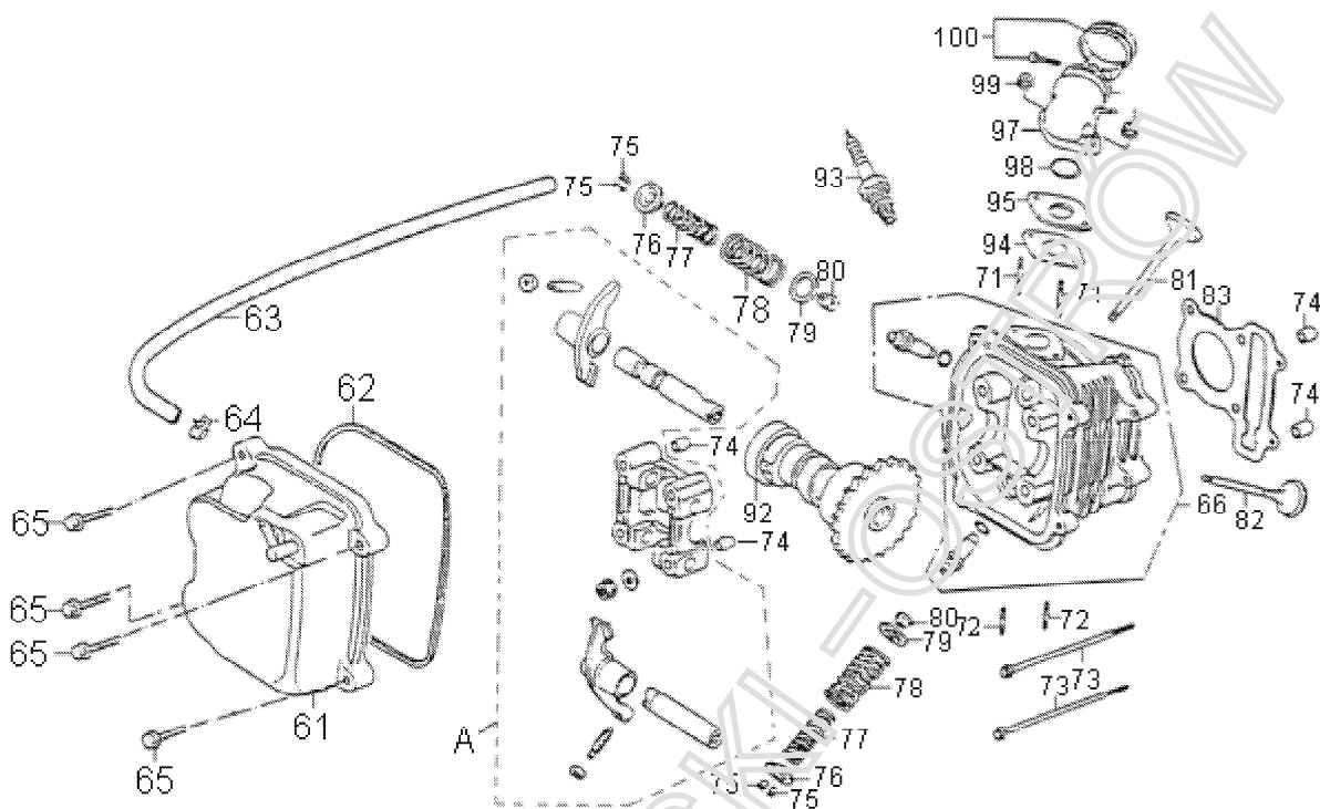
FIG2 CYLINDER HEAD COVER.CYLINDER HEAD
