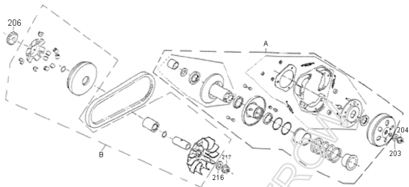
FIG.7 DRIVEN PULLEY
