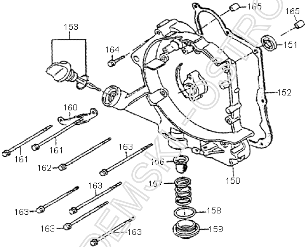
FIG.4 RIGHT CRANKCASE COVER
