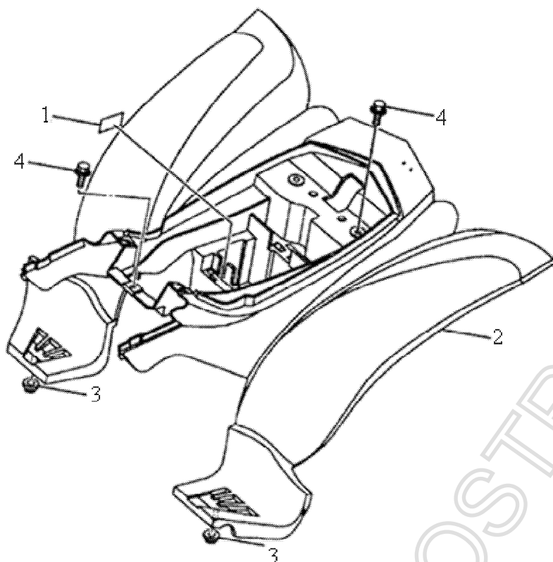
FIG.12 REAR FENDER
