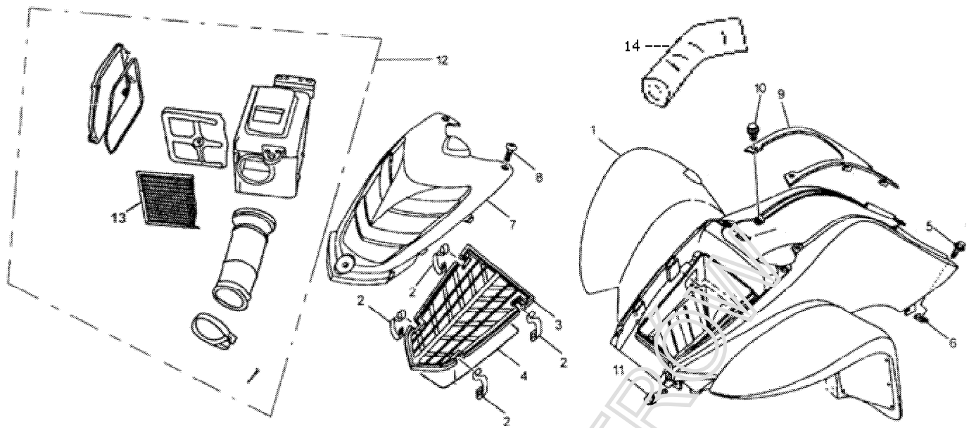
FIG.11 FRONT FENDER
